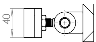
DETAIL B SCALE 1 : 3
