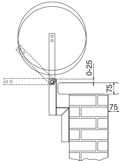
Coping stone bracket
