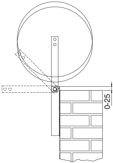
Wall fixing bracket
