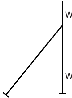
END POST 1 x Strut 2 x Winders 1 x Stretcher bar 2 x M8 x 40 bolts 1 x M8 x 25 bolts 5 x M8 bolts
