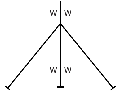
CORNER POST 2 x Strut 4 x Winders 2 x Stretcher bar 4 x M8 x 40 bolts 2 x M8 x 25 bolts 10 x M8 bolts
