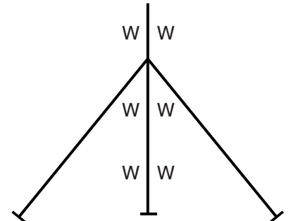
CORNER POST 2 x Strut 6 x Winders 2 x Stretcher bar 6 x M8 x 40 bolts 2 x M8 x 25 bolts 14 x M8 bolts
