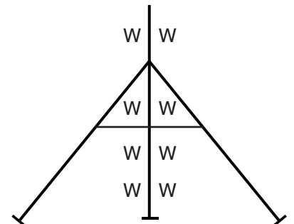
CORNER POST 2 x Strut 2 x Brace 8 x Winders 2 x Stretcher bar 8 x M8 x 40 bolts 6 x M8 x 25 bolts 22 x M8 bolts
