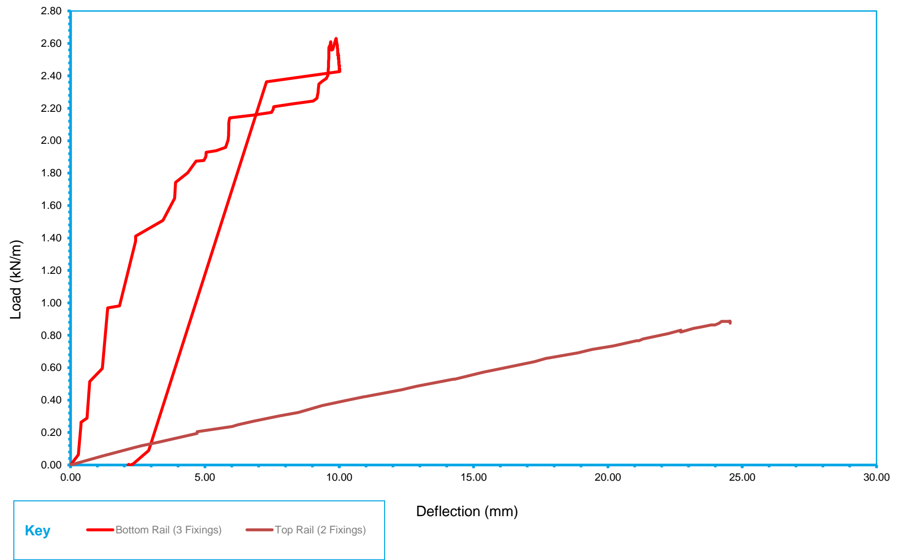
Chart 1 - Load Deflection Curves for Load Testing of FH Brundle's 2400 mm Elegance Juliet Balcony Rail With No Glass
